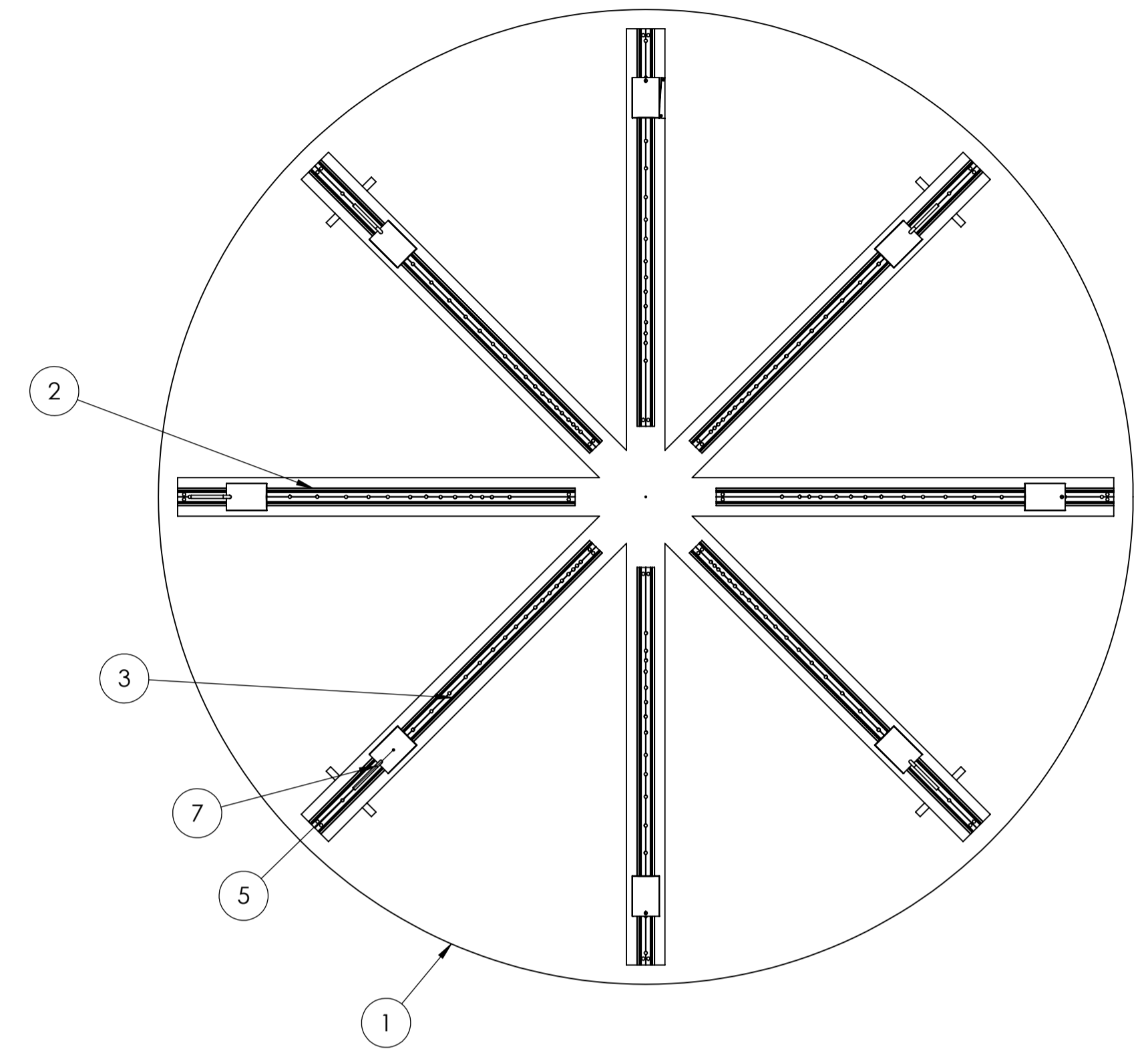
TOP VIEW
