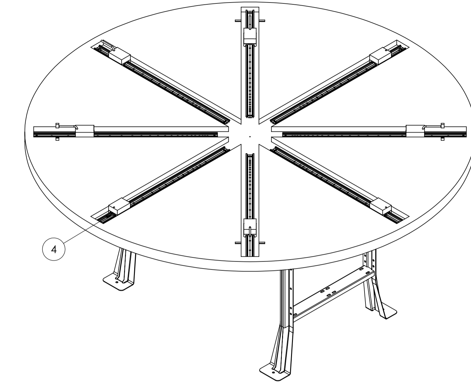
ISOMETRIC VIEW
